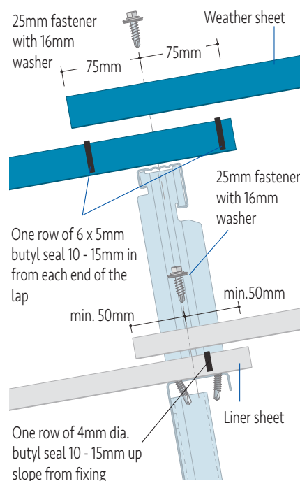
End lap fixing details - roof profiles
