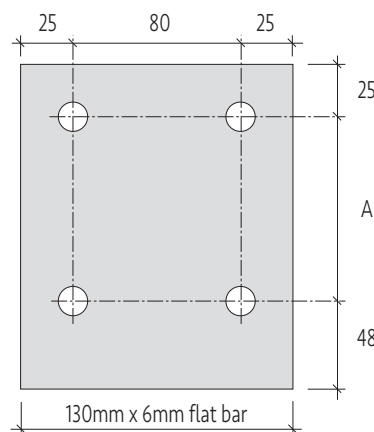
Welded Cleats
