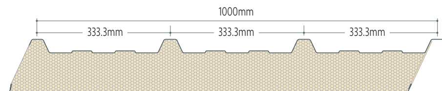
Trapezoidal roof & wall panel dimensions
