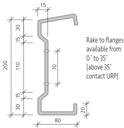
Cleat section depth
